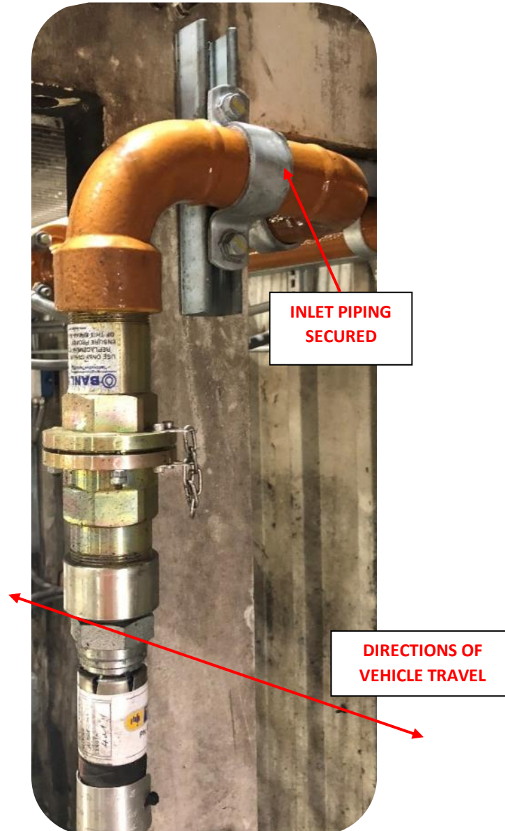
Figure 11 - Example of BAV Installation
