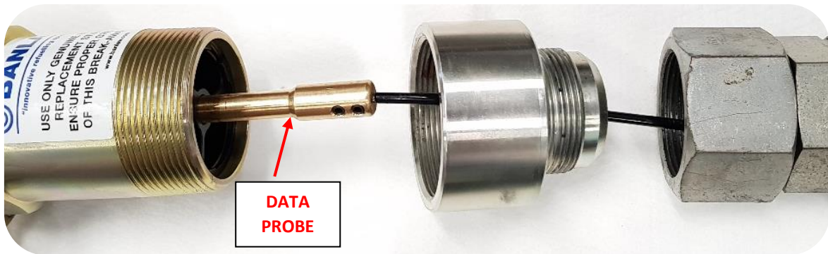
Figure 24 - Data Cable Secured into BAV Outlet Probe
