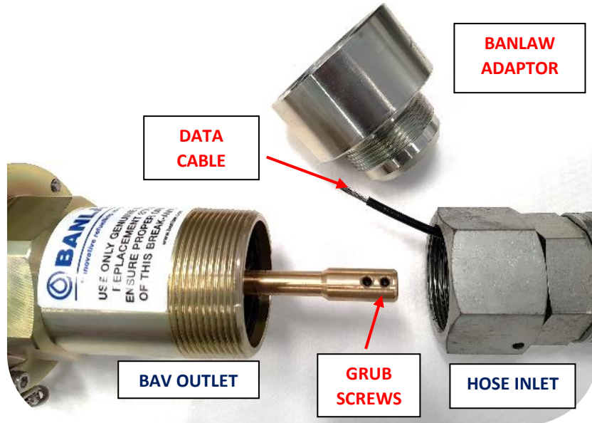
Figure 23 - Parts Connecting FuelTrack BAV Outlet into Dispensing Hose
