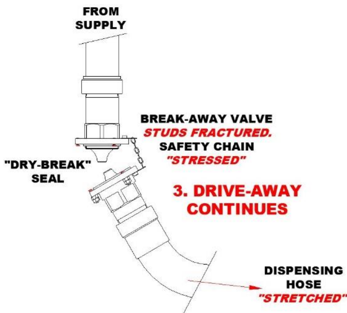
Figure 14 - Initial BAV Separation
