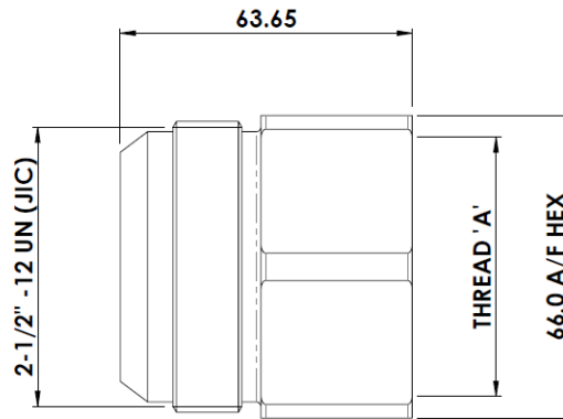
Figure 16 – 3" pipe threads to 2-1/2" JIC(M) adaptor details
