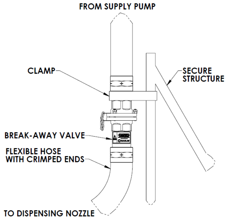
Figure 9 – Basic Arrangement of a BAV Installation
