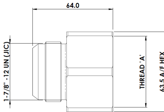
Figure 17 – 2" pipe threads to 2-1/2" JIC(M) adaptor details
