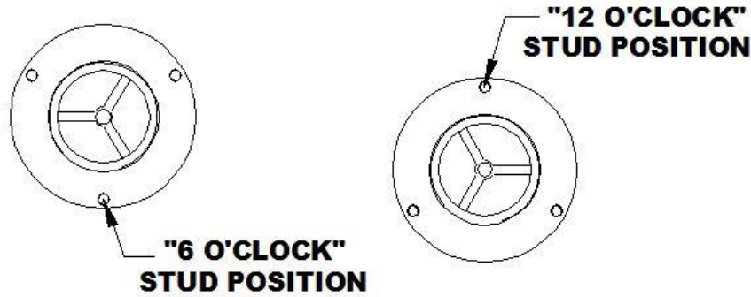
Figure 6 - Illustration of BAV Stud Position (end view of BAV)
