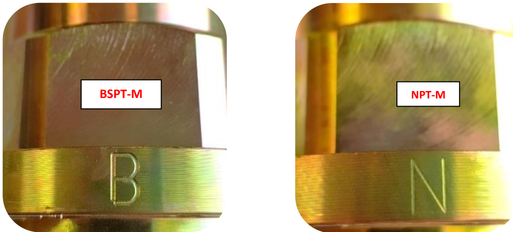
Figure 5 - Marking for Thread Type
