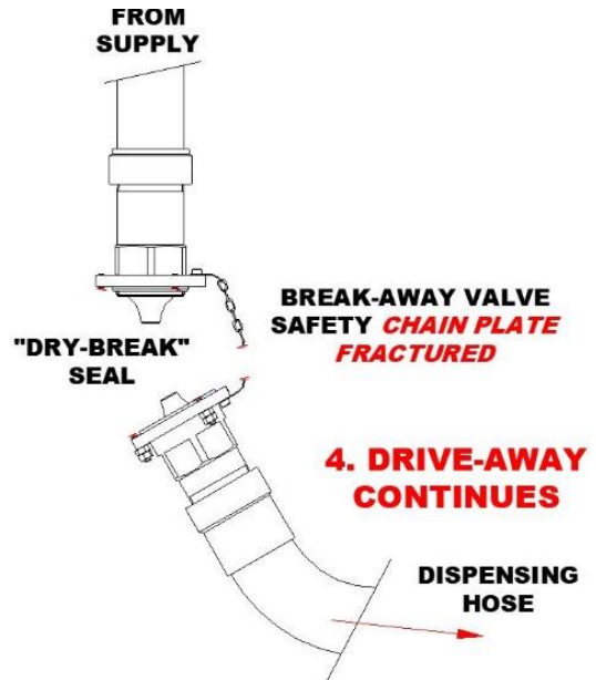
Figure 15 - Complete BAV Separation
