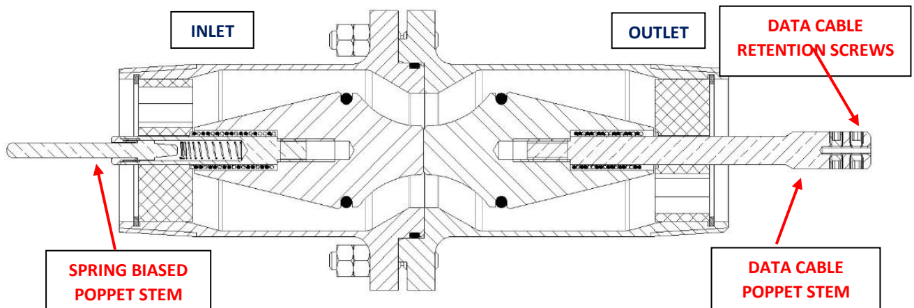
Figure 20 - Sectioned View of Banlaw FuelTrack BAV (R2 version shown)
