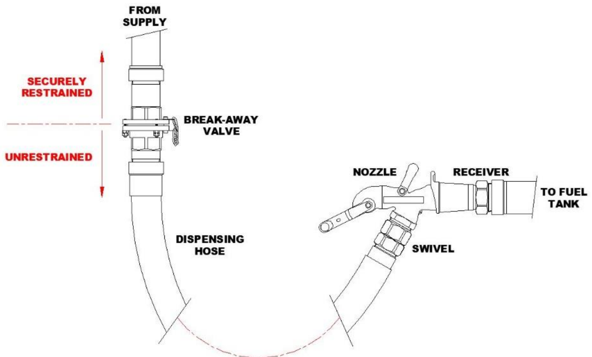
Figure 10 - Example of a Refuelling System
