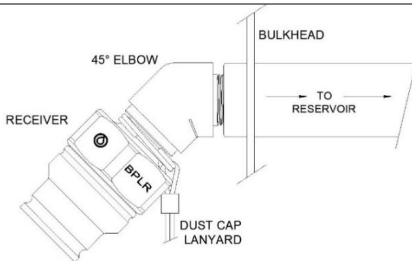
Figure 7 - Example of a BPL Receiver with Elbow
