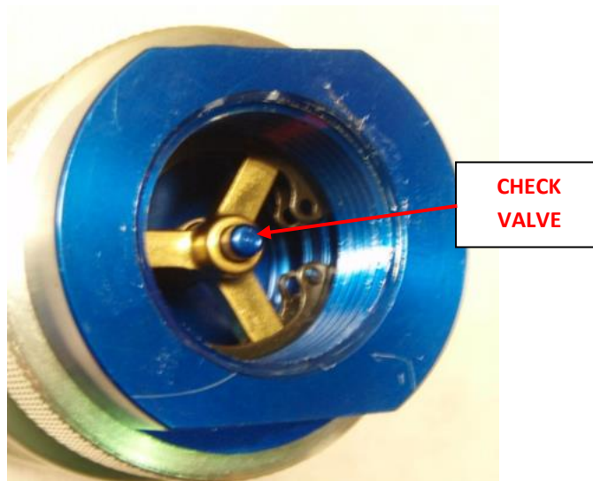
Figure 13 - Rear (Outlet) of Evacuation Coupling showing Internal Check Valve (Closed)
