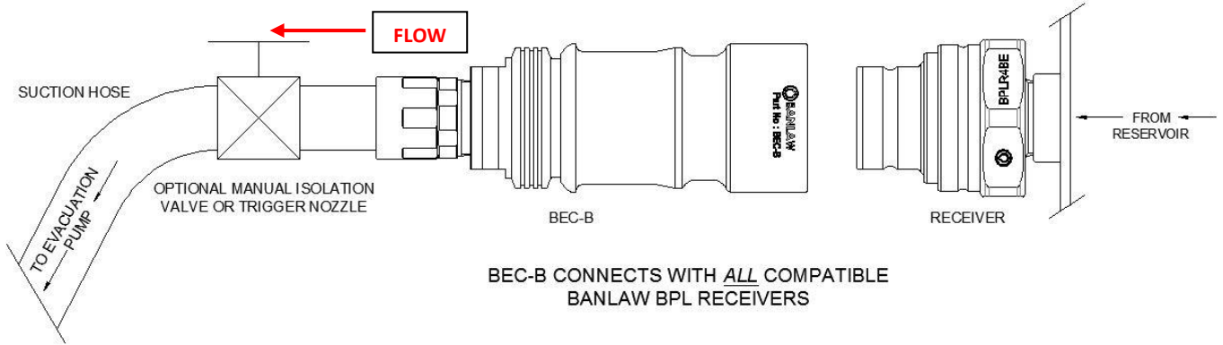
Figure 6 - Example of a waste fluid evacuation system using the BEC-B
