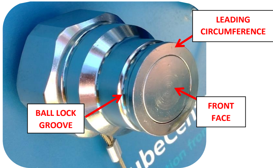
Figure 10 - Critical Areas of Damage on GTXR Receivers
