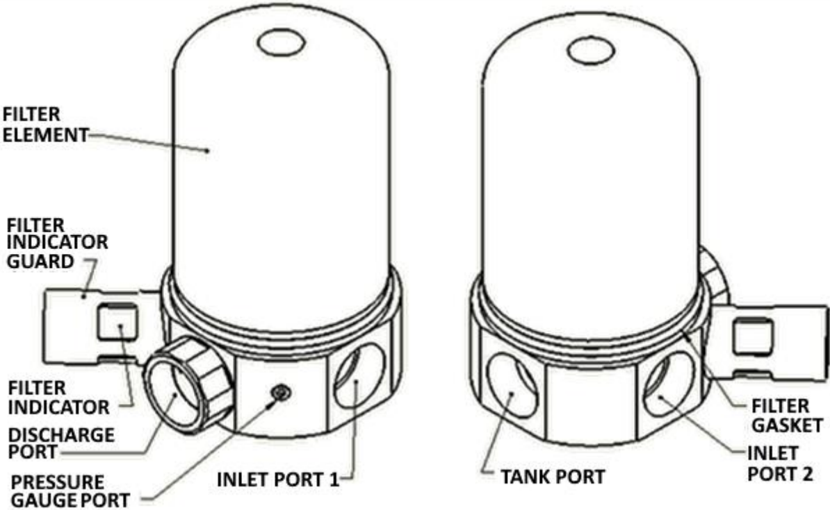
Figure 2 – External Features
