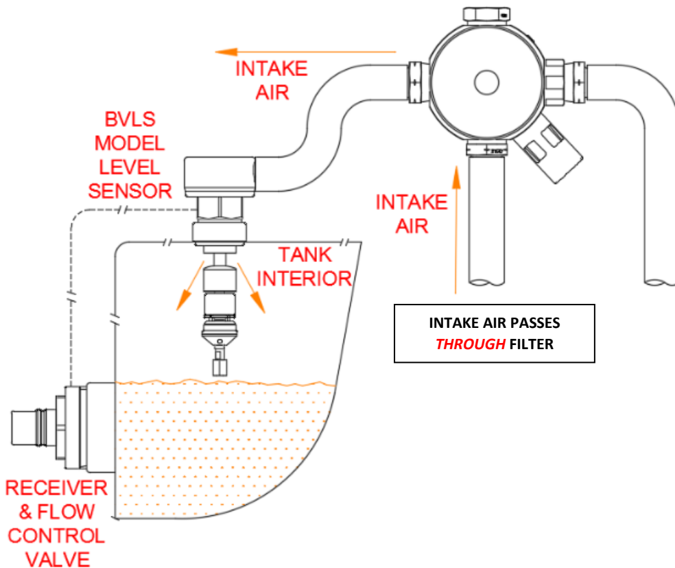
Figure 8 – Air Intake
