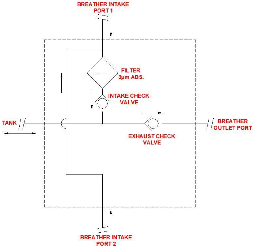
Figure 3 - Basic Flow Schematic of Breather
