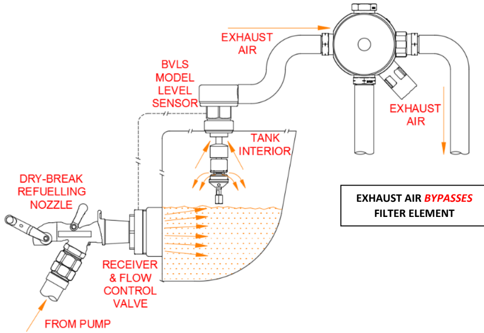
Figure 7 – Tank Refilling (Air Exhaust)
